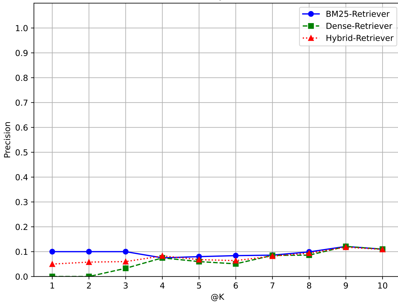
Query 22
